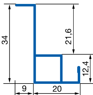
Randprofil Omega 34 mm L = 6.00 m
